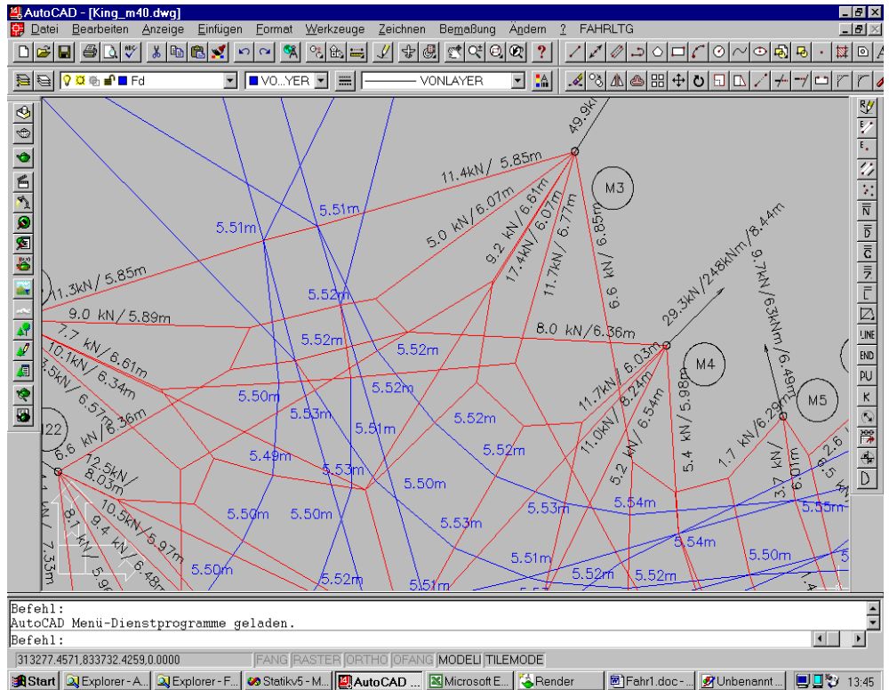
Pic.7 : Wire forces and height of contact line at -40 °C
