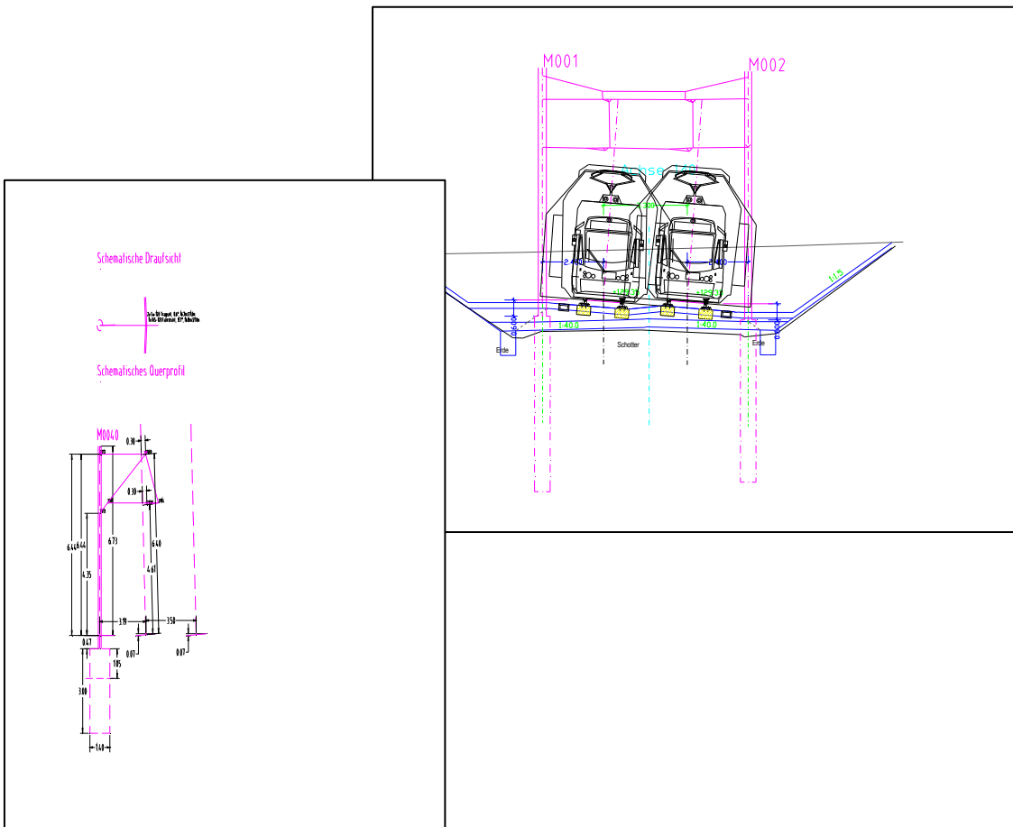
Pic.11 : Cross sections with cantilever and cross span construction
