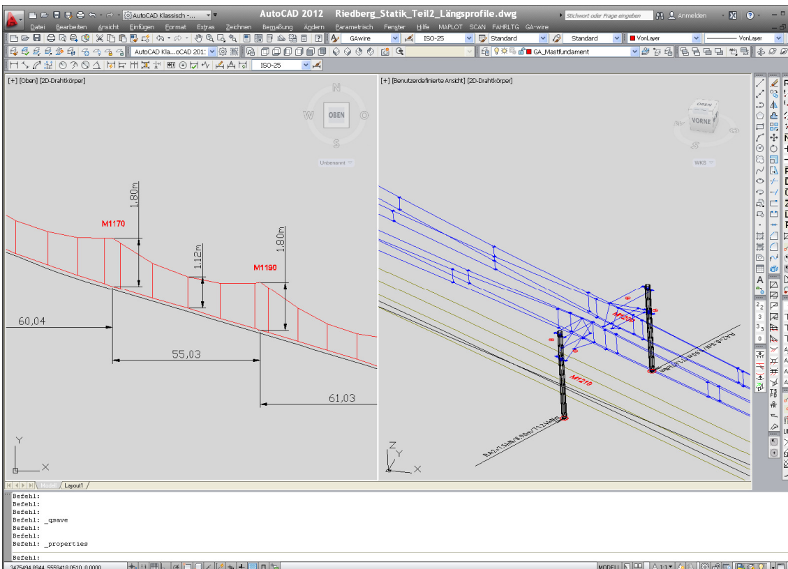
Pic.5 : Longitudinal profiles of catenary with droppers
