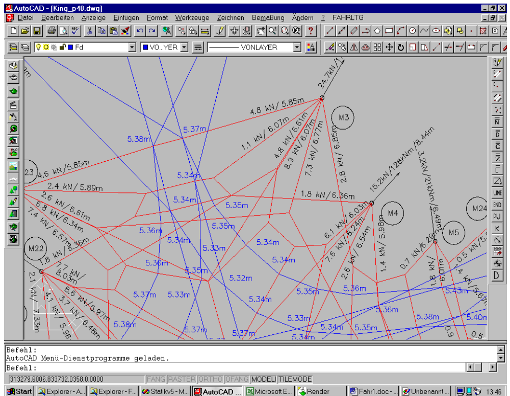
Pic.8 : Wire forces and height of contact line at + 40 °C
